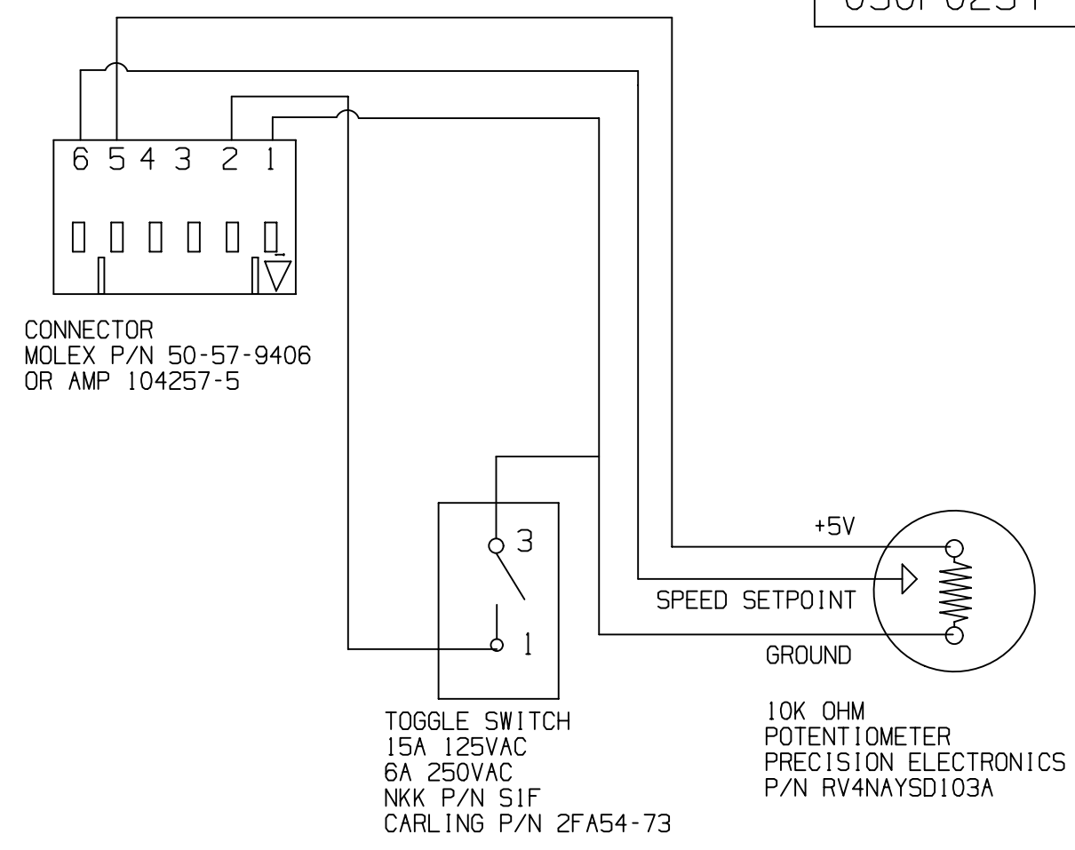
WIRING DIAGRAM
